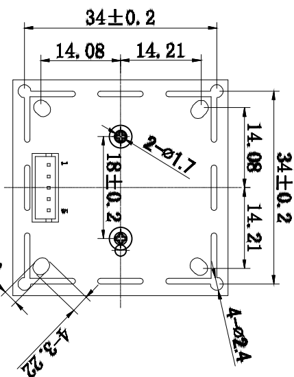
FIG. 5, Top entry type, B-PIN DESIGNED BY DM US85V P1N6 P1N4 P1N8 P1N2 P1N1
